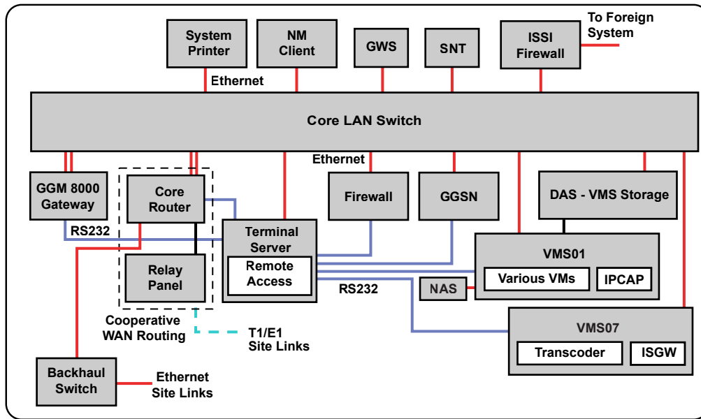
Figure 2: Master Site with HPD Overlay – Single Zone Redundant Configuration
