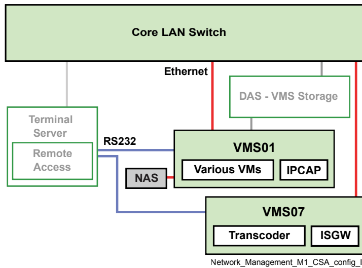
Figure 7: Network Management Subsystem – Single Zone Non-Redundant Configuration
