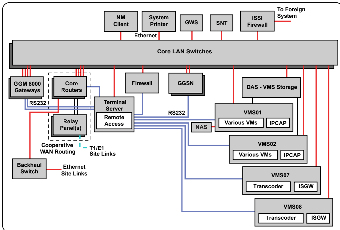
Figure 2: Master Site with HPD Overlay – Single Zone Redundant Configuration
