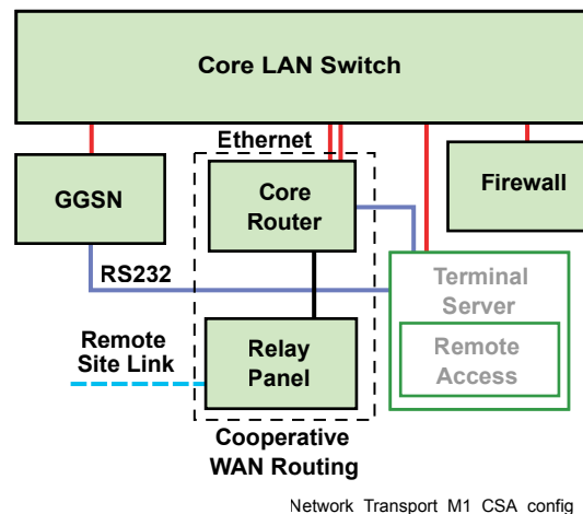
Figure 10: Network Transport Subsystem – Single Zone Non-Redundant Configuration
