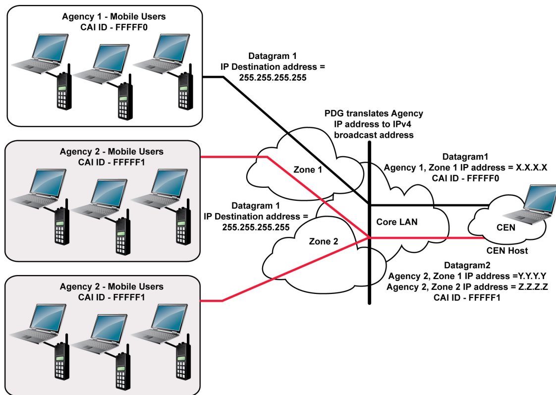
Figure 6: Broadcast Messaging in a Multi-Zone System
