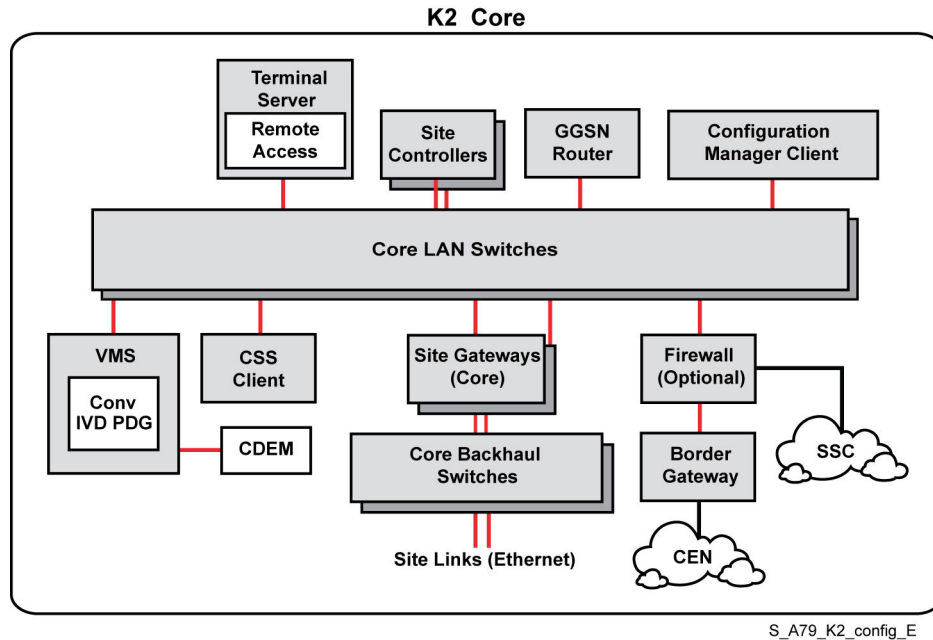
Figure 4: ASTRO 25 Conventional with Integrated Data Architecture for K Core Systems
