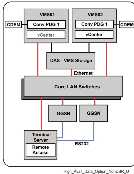
Figure 2: Data Subsystem – HA Data – Non-DSR
